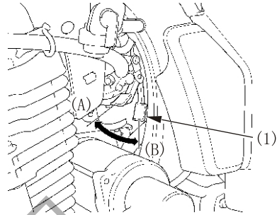
(1)阻风门手柄 (A)全闭 (B)全开
